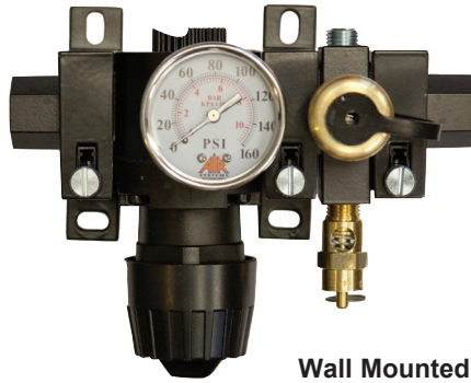
Wall Mounted Point of Attachment POA-1WM
