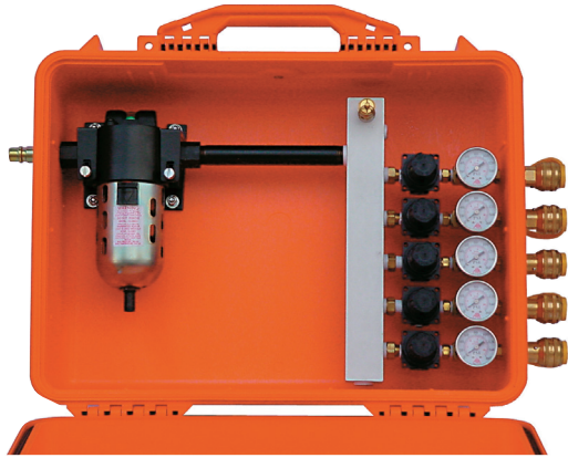
Portable Point of Attachment POA-5RF
